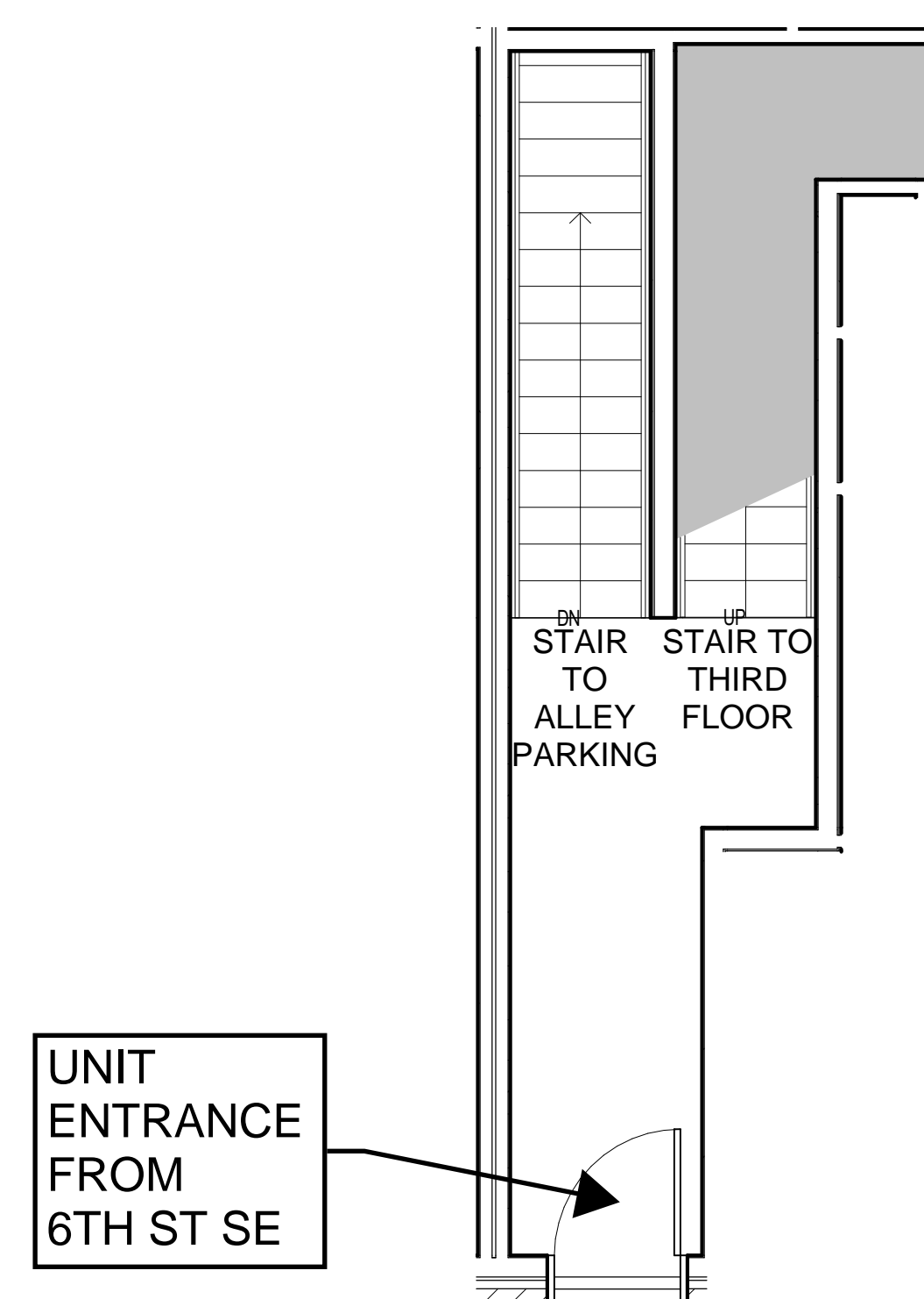
SECOND FLOOR PLAN- 4 BEDROOM TOWNHOME
