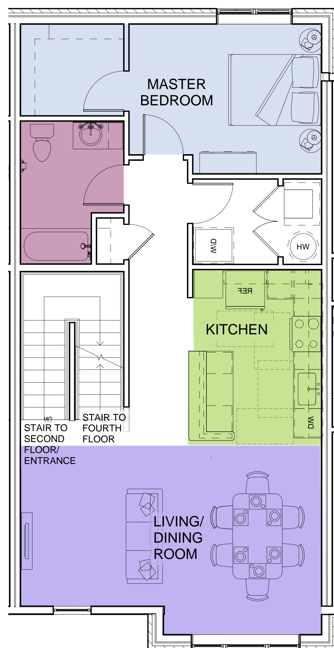
THIRD FLOOR PLAN - 4 BEDROOM TOWNHOME
