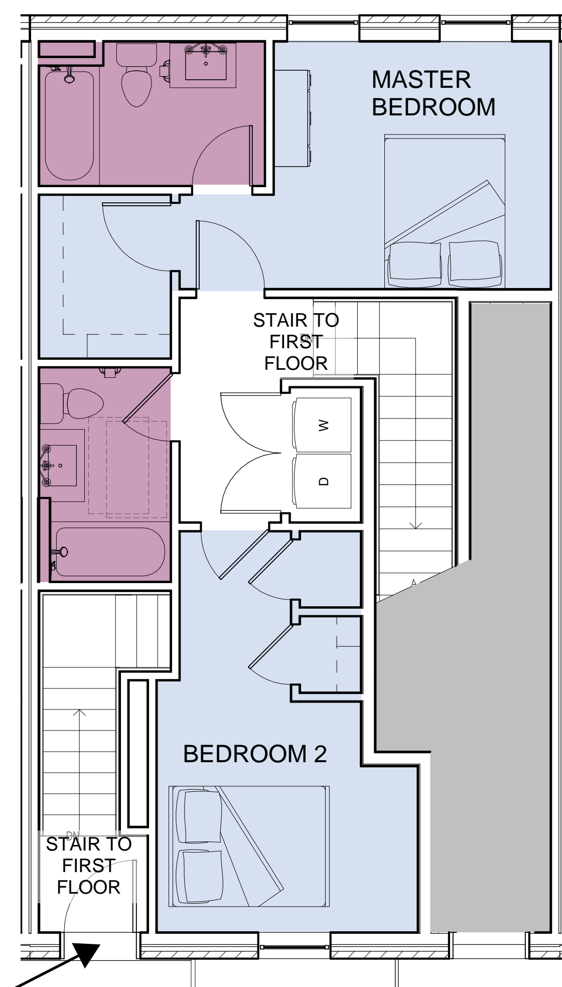
SECOND FLOOR PLAN - 2 BEDROOM TOWNHOME
